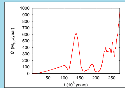
Mass accretion for delayed feedback.
