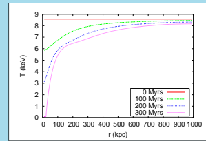
Temperature profile for pure cooling.
