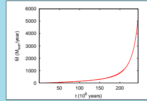
Mass accretion for pure cooling.
