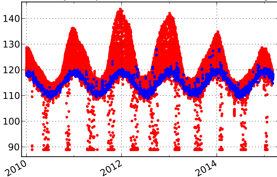
Solar array temps at off-nominal roll 5 - 10 degrees
