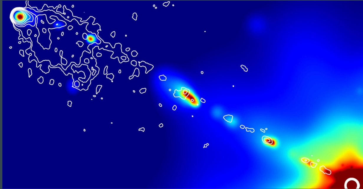
3C 111 - jet clearly shows X-ray first offsets (Clautice et al. 2016)
