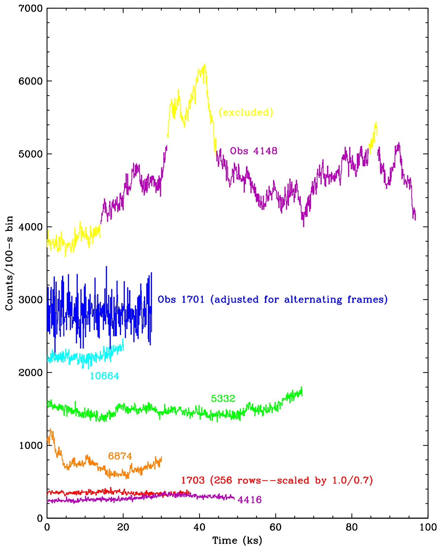
Lightcurves, S2+S3 only, |tg\_d| < 0.001 , |\lambda| > 2 \text{ \AA}
