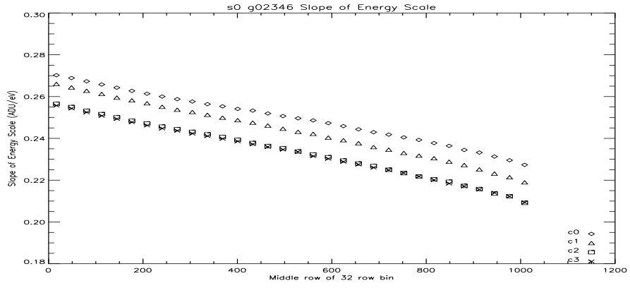
Figure 70: S0 Slope of the Energy Scale Vs Row at -110C.
