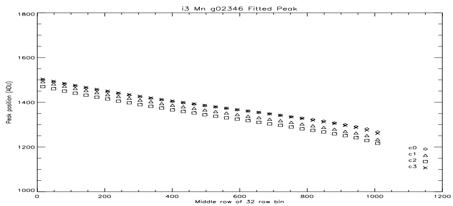
Figure 13: i3 Mn Peak Vs Row at -110C.
