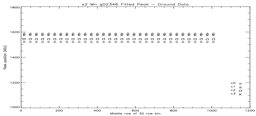
Figure 112: S2 Mn Peak Vs Row at -110C.
