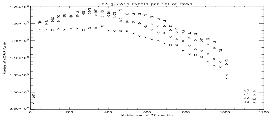
Figure 89: S3 ASCA G02346 Counts Vs Row at -110C.
