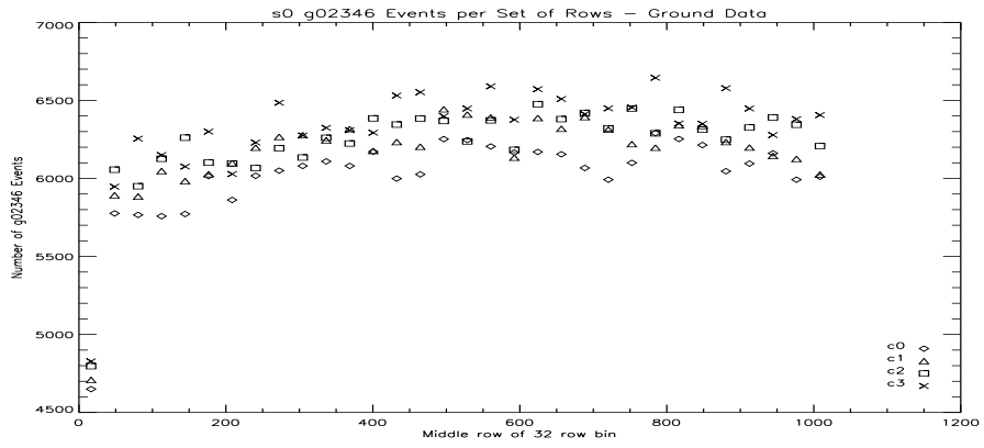
Figure 176: S0 ASCA G02346 Counts Vs Row at -110C.
