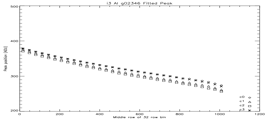
Figure 11: i3 Al Peak Vs Row at -110C.
