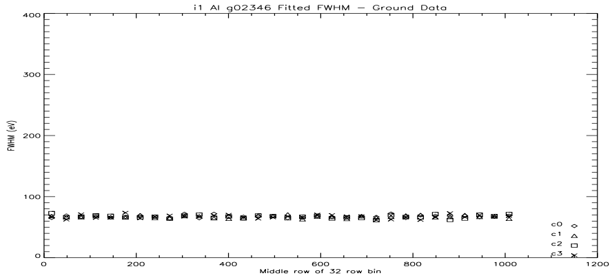
Figure 125: i1 Al FWHM Vs Row at -110C.
