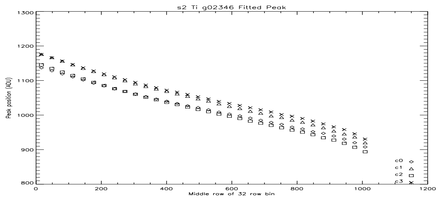
Figure 21: S2 Ti Peak Vs Row at -110C.
