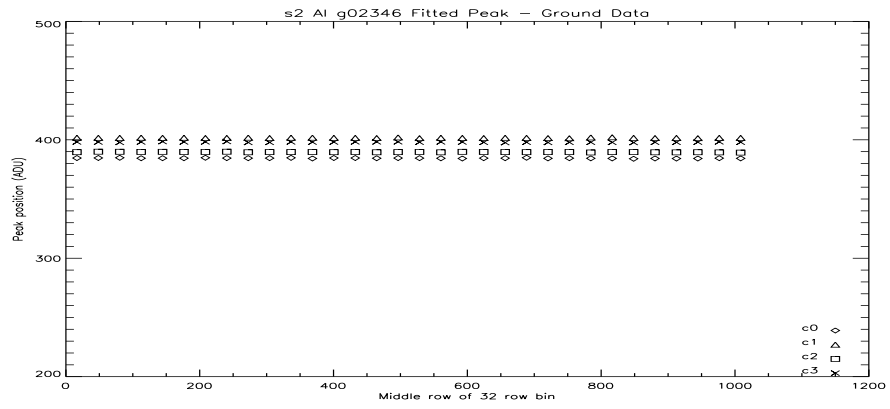
Figure 110: S2 Al Peak Vs Row at -110C.
