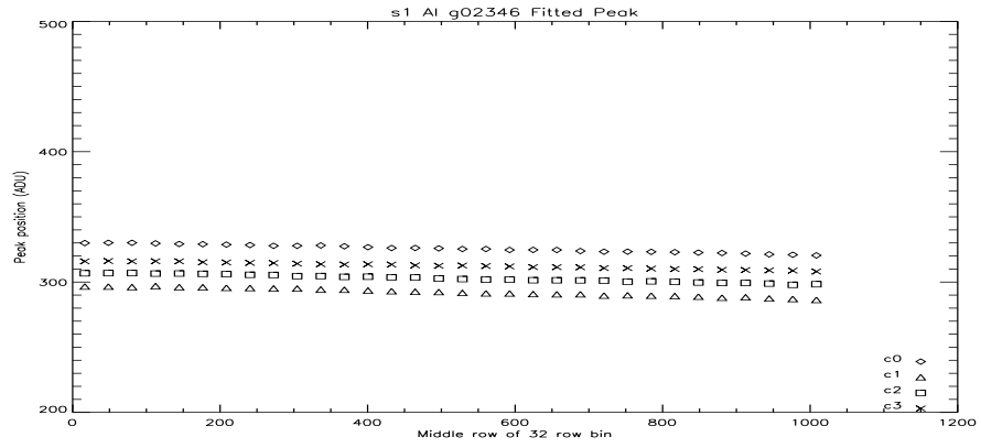
Figure 17: S1 Al Peak Vs Row at -110C.
