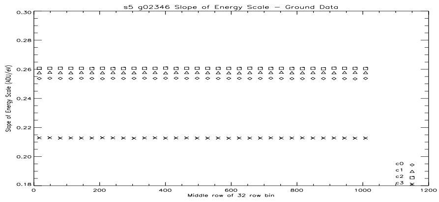
Figure 170: S5 Slope of the Energy Scale Vs Row at -110C.
