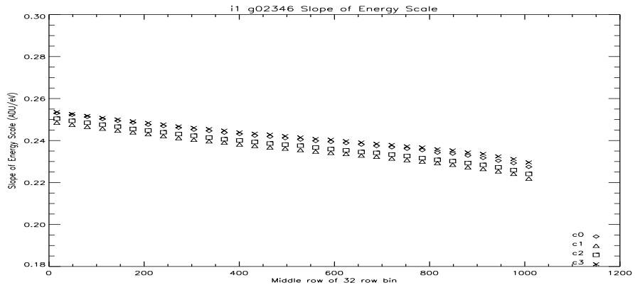
Figure 64: i1 Slope of the Energy Scale Vs Row at -110C.
