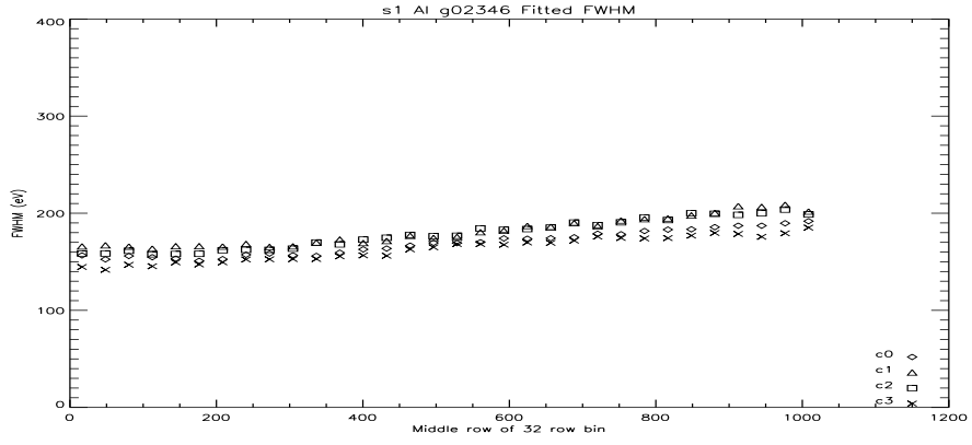
Figure 47: S1 Al FWHM Vs Row at -110C.
