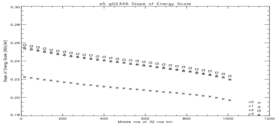
Figure 80: S5 Slope of the Energy Scale Vs Row at -110C.
