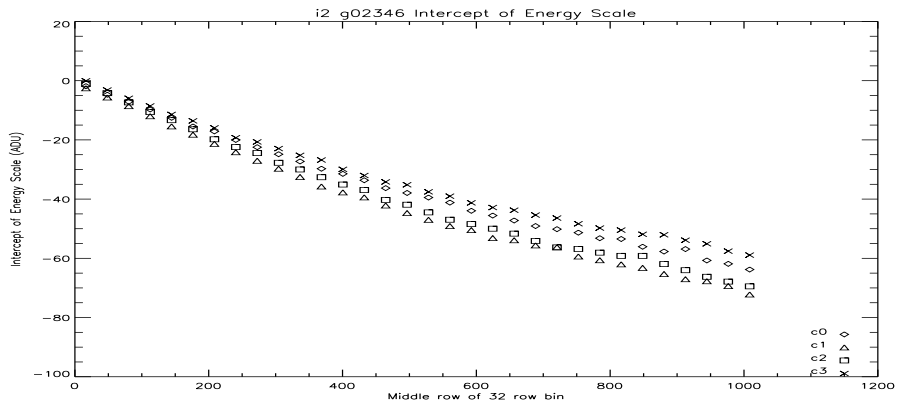
Figure 67: i2 Intercept of the Energy Scale Vs Row at -110C.
