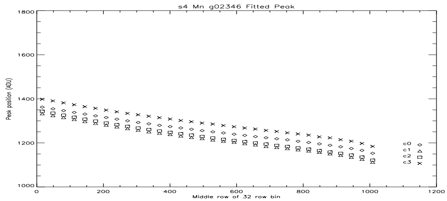
Figure 28: S4 Mn Peak Vs Row at -110C.
