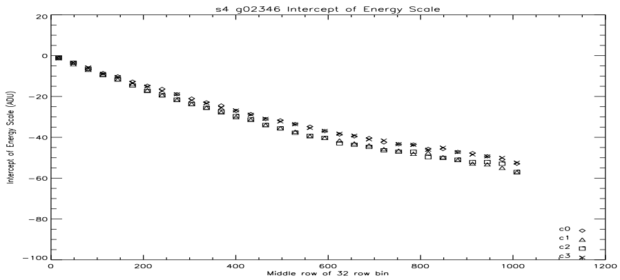
Figure 79: S4 Intercept of the Energy Scale Vs Row at -110C.
