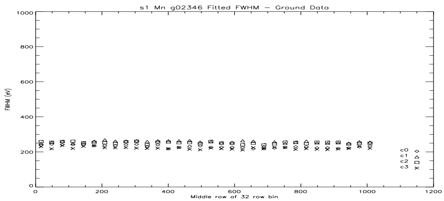
Figure 139: S1 Mn FWHM Vs Row at -110C.
