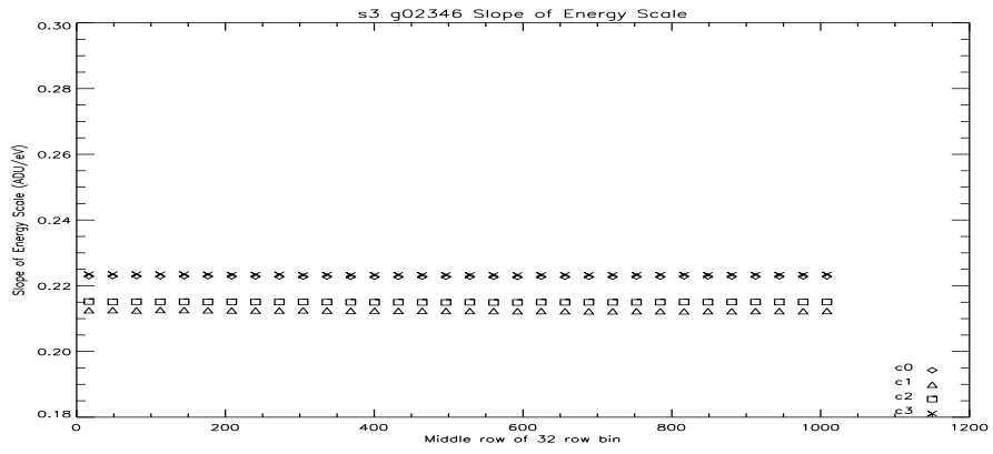
Figure 76: S3 Slope of the Energy Scale Vs Row at -110C.
