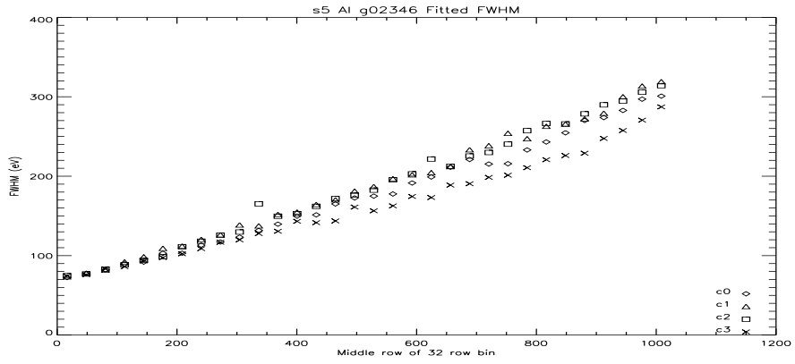
Figure 59: S5 Al FWHM Vs Row at -110C.
