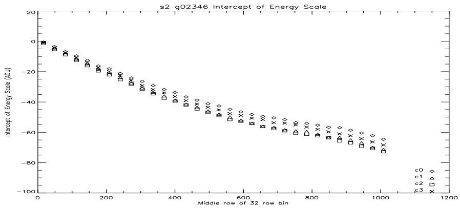
Figure 75: S2 Intercept of the Energy Scale Vs Row at -110C.
