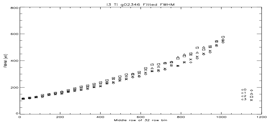
Figure 42: i3 Ti FWHM Vs Row at -110C.
