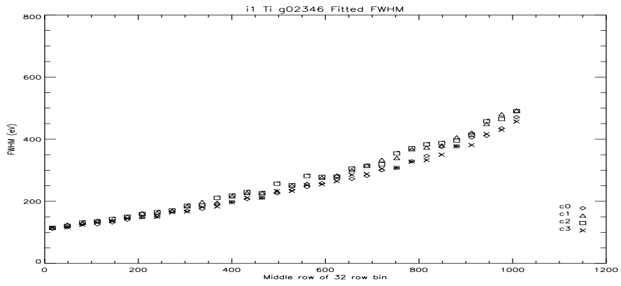
Figure 36: i1 Ti FWHM Vs Row at -110C.
