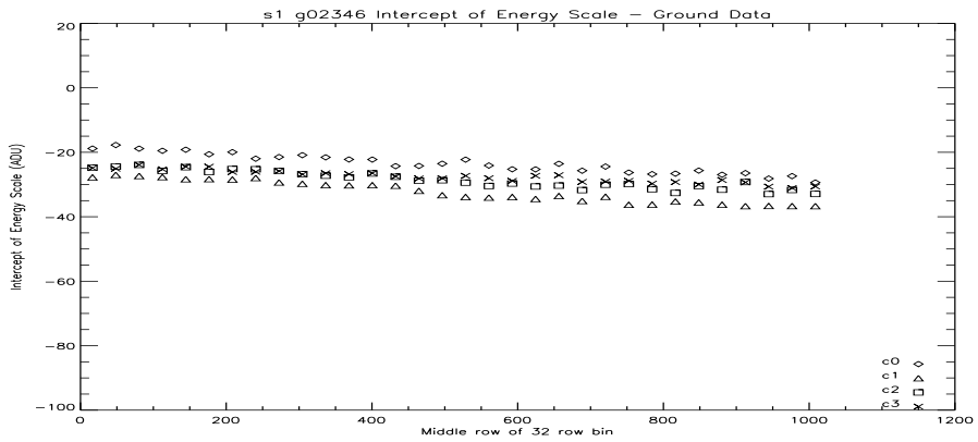
Figure 163: S1 Intercept of the Energy Scale Vs Row at -110C.
