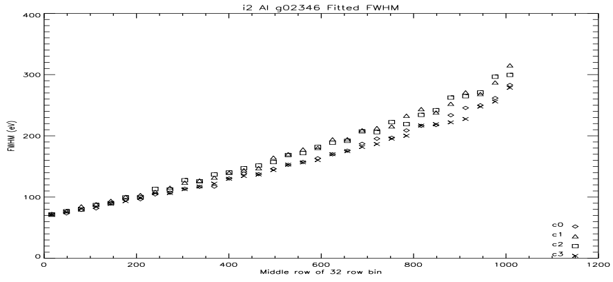
Figure 38: i2 Al FWHM Vs Row at -110C.
