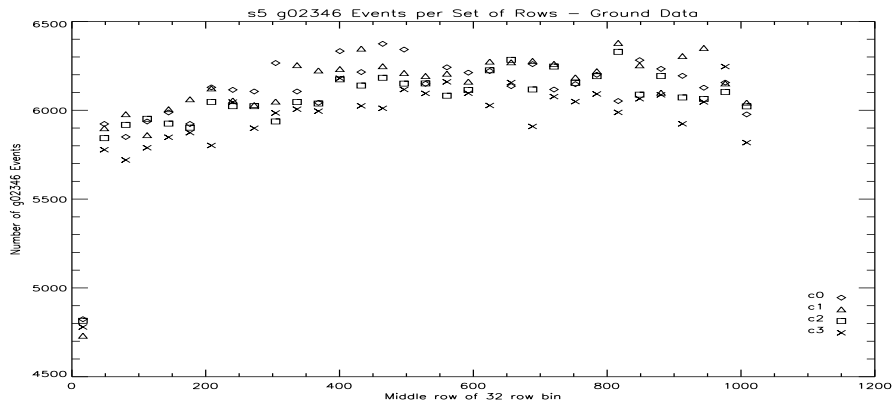
Figure 181: S5 ASCA G02346 Counts Vs Row at -110C.
