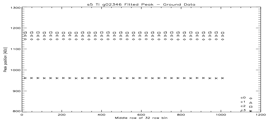
Figure 120: S5 Ti Peak Vs Row at -110C.
