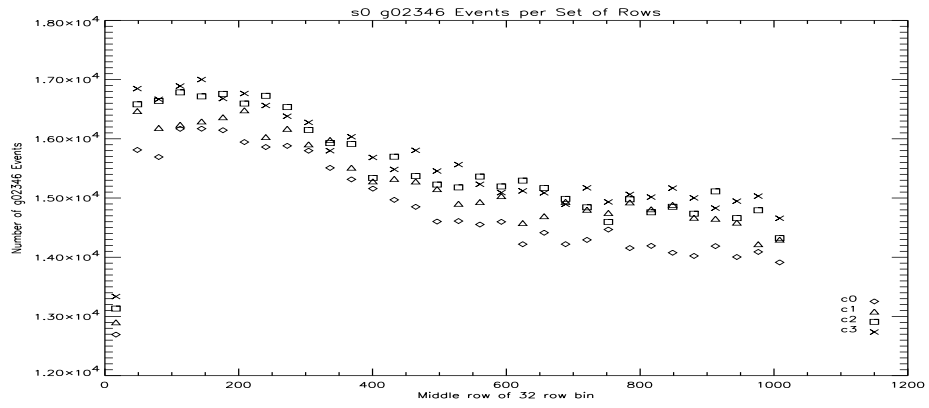
Figure 86: S0 ASCA G02346 Counts Vs Row at -110C.
