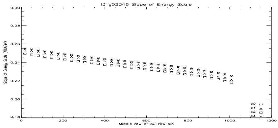
Figure 68: i3 Slope of the Energy Scale Vs Row at -110C.
