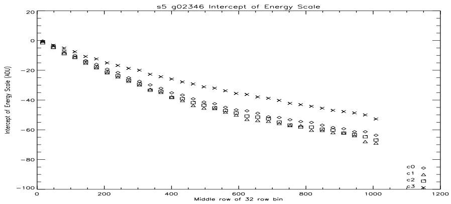
Figure 81: S5 Intercept of the Energy Scale Vs Row at -110C.
