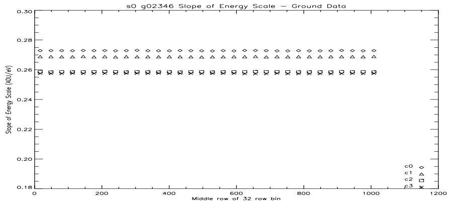
Figure 160: S0 Slope of the Energy Scale Vs Row at -110C.
