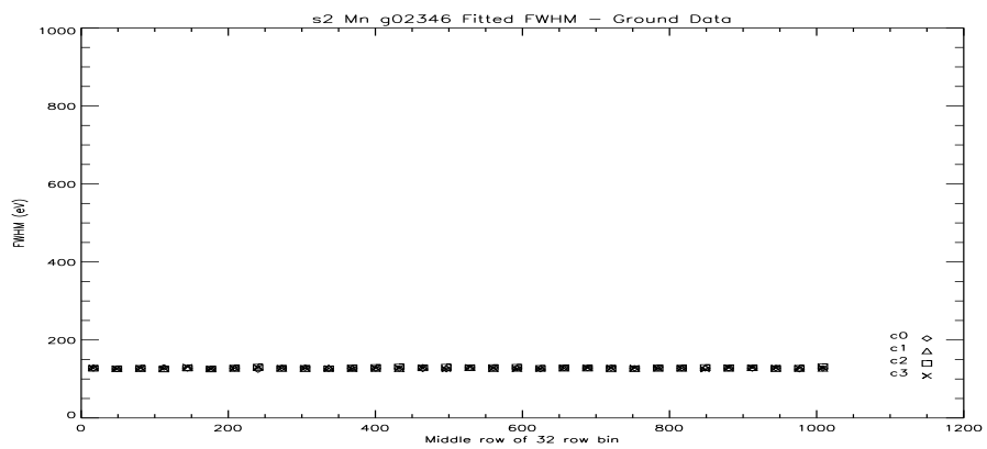
Figure 142: S2 Mn FWHM Vs Row at -110C.
