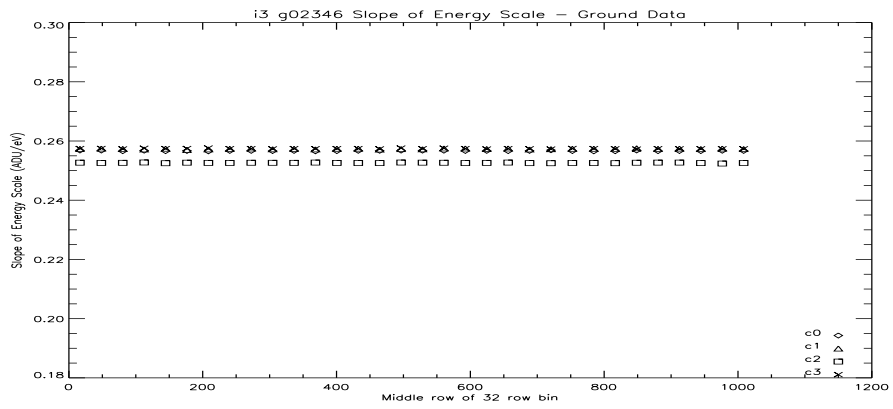
Figure 158: i3 Slope of the Energy Scale Vs Row at -110C.
