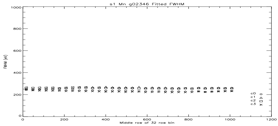
Figure 49: S1 Mn FWHM Vs Row at -110C.
