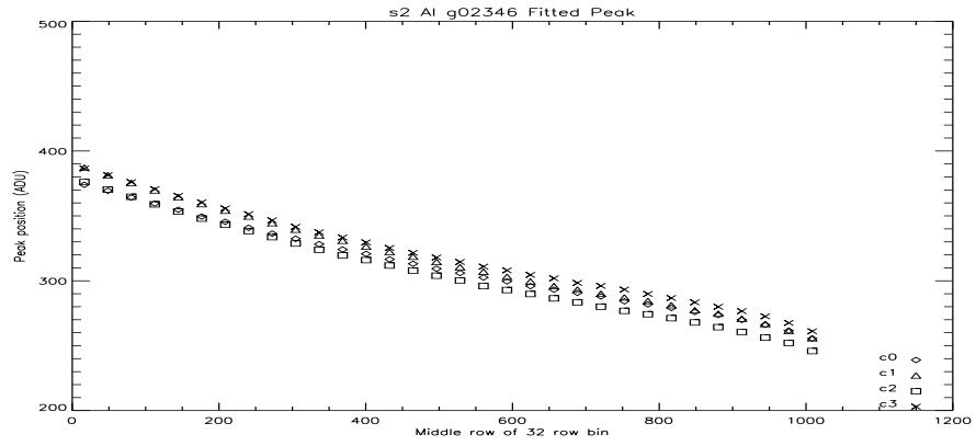
Figure 20: S2 Al Peak Vs Row at -110C.
