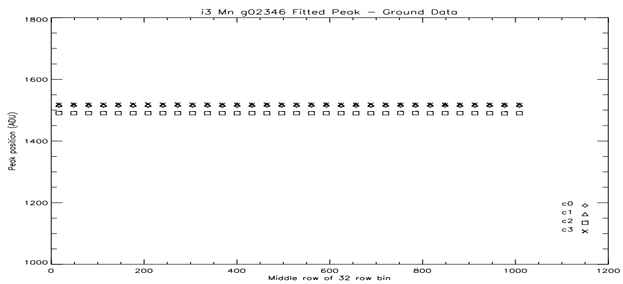
Figure 103: i3 Mn Peak Vs Row at -110C.
