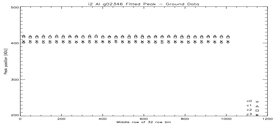
Figure 98: i2 Al Peak Vs Row at -110C.
