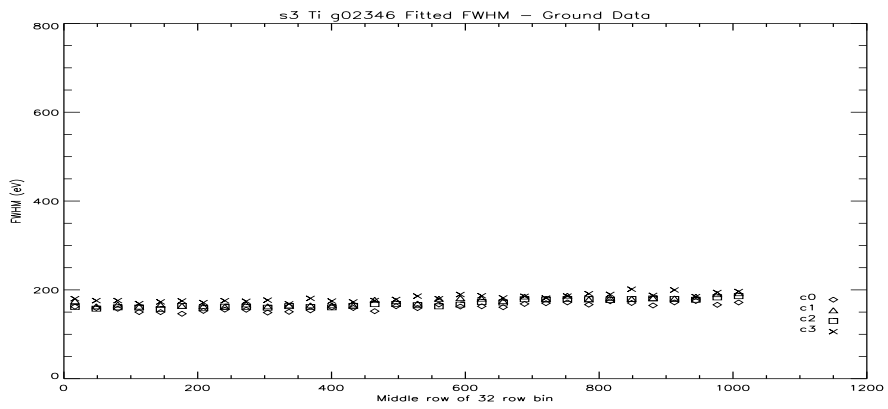
Figure 144: S3 Ti FWHM Vs Row at -110C.
