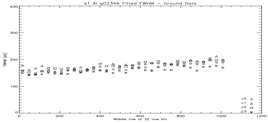
Figure 137: S1 Al FWHM Vs Row at -110C.
