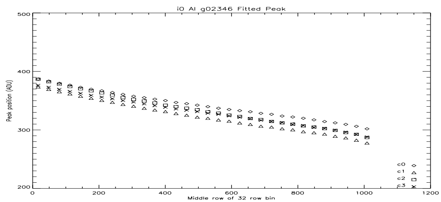
Figure 2: i0 Al Peak Vs Row at -110C.
