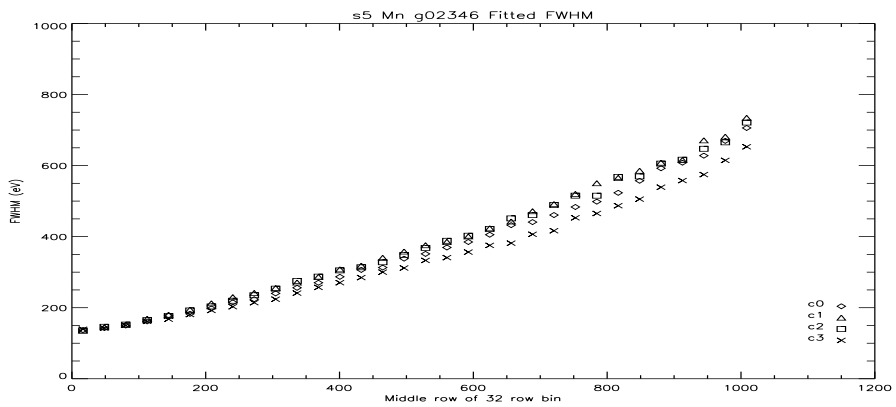
Figure 61: S5 Mn FWHM Vs Row at -110C.
