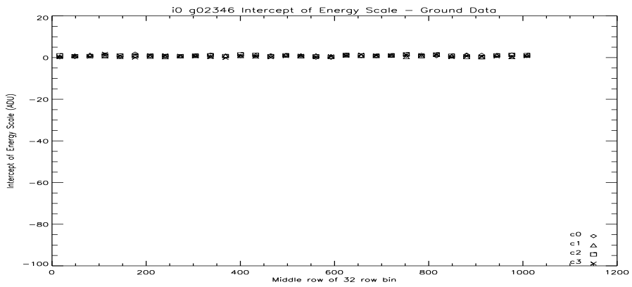
Figure 153: i0 Intercept of the Energy Scale Vs Row at -110C.
