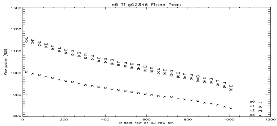
Figure 30: S5 Ti Peak Vs Row at -110C.
