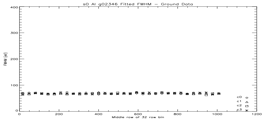
Figure 134: S0 Al FWHM Vs Row at -110C.
