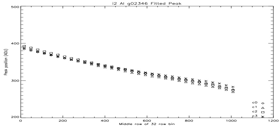
Figure 8: i2 Al Peak Vs Row at -110C.
