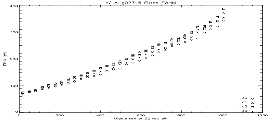
Figure 50: S2 Al FWHM Vs Row at -110C.
