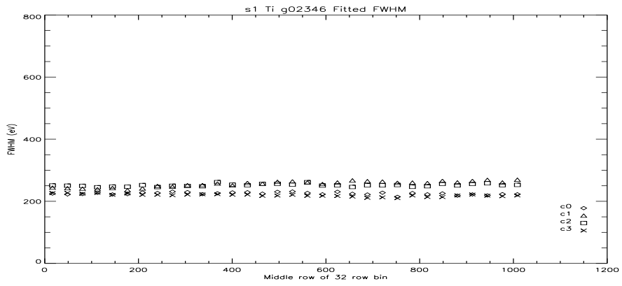
Figure 48: S1 Ti FWHM Vs Row at -110C.
