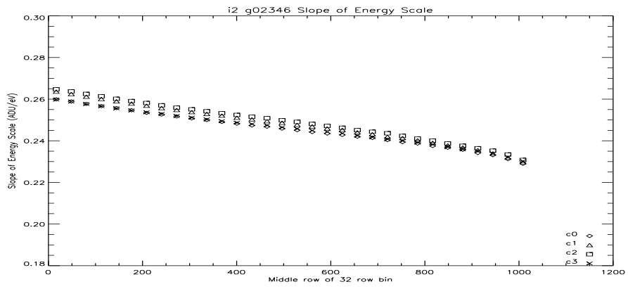
Figure 66: i2 Slope of the Energy Scale Vs Row at -110C.
