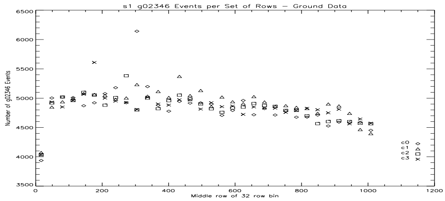
Figure 177: S1 ASCA G02346 Counts Vs Row at -110C.
