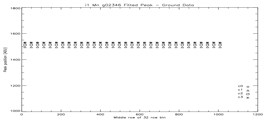
Figure 97: i1 Mn Peak Vs Row at -110C.
