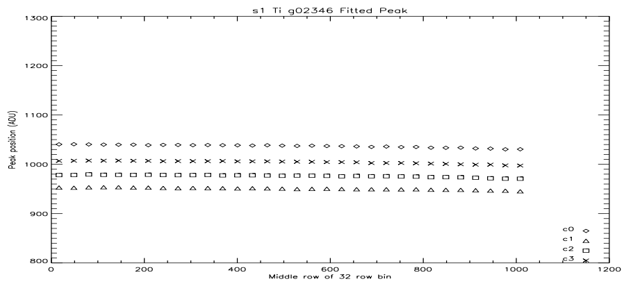
Figure 18: S1 Ti Peak Vs Row at -110C.
