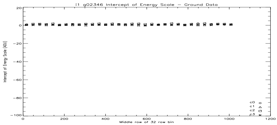
Figure 155: i1 Intercept of the Energy Scale Vs Row at -110C.
