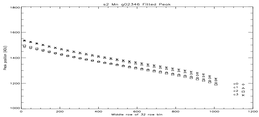
Figure 22: S2 Mn Peak Vs Row at -110C.
