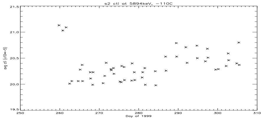
Figure 1: s2 Average CTI at -110C.
