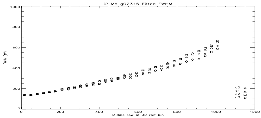
Figure 40: i2 Mn FWHM Vs Row at -110C.
