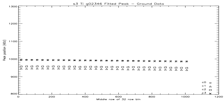
Figure 114: S3 Ti Peak Vs Row at -110C.
