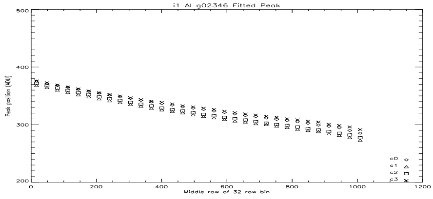
Figure 5: i1 Al Peak Vs Row at -110C.
