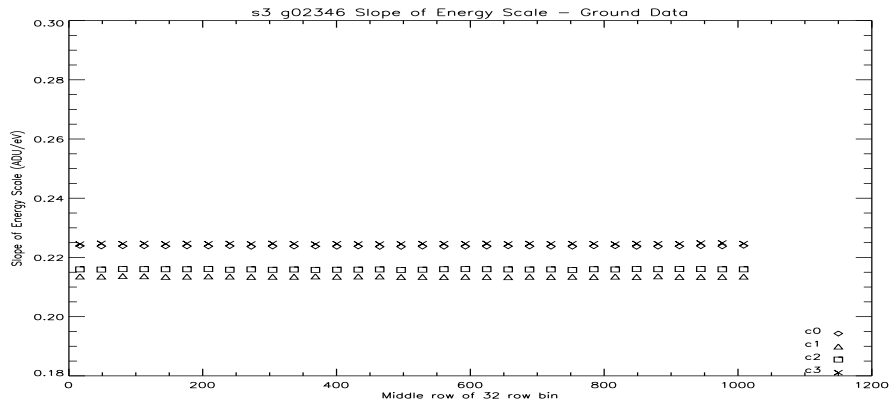
Figure 166: S3 Slope of the Energy Scale Vs Row at -110C.
