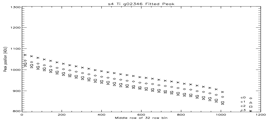
Figure 27: S4 Ti Peak Vs Row at -110C.
