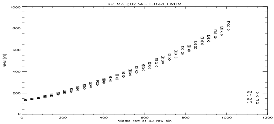
Figure 52: S2 Mn FWHM Vs Row at -110C.
