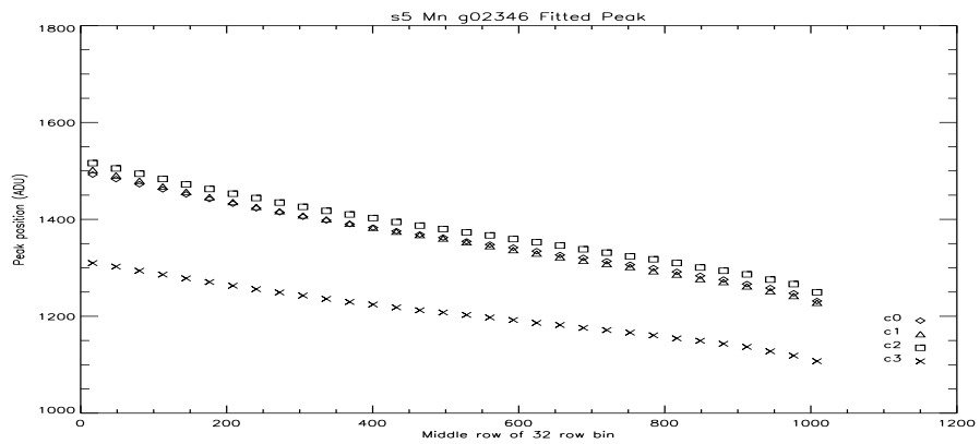
Figure 31: S5 Mn Peak Vs Row at -110C.
