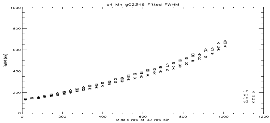
Figure 58: S4 Mn FWHM Vs Row at -110C.
