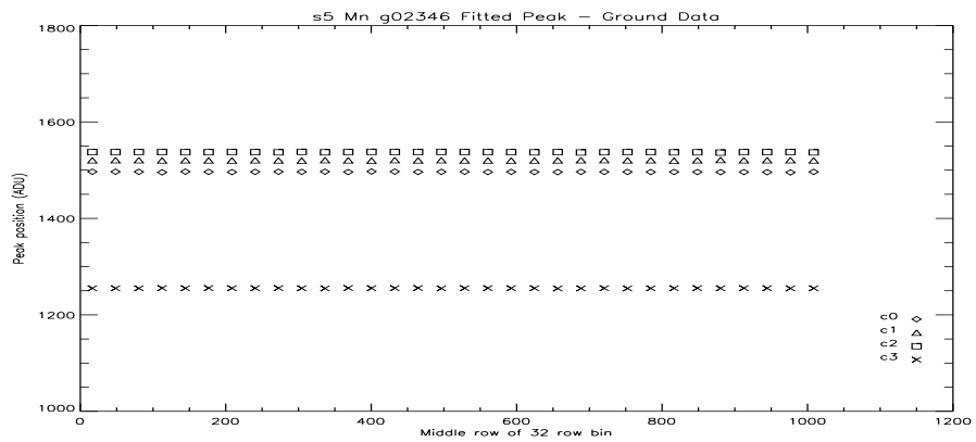
Figure 121: S5 Mn Peak Vs Row at -110C.
