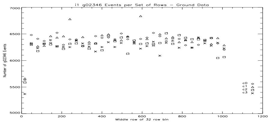
Figure 173: i1 ASCA G02346 Counts Vs Row at -110C.
