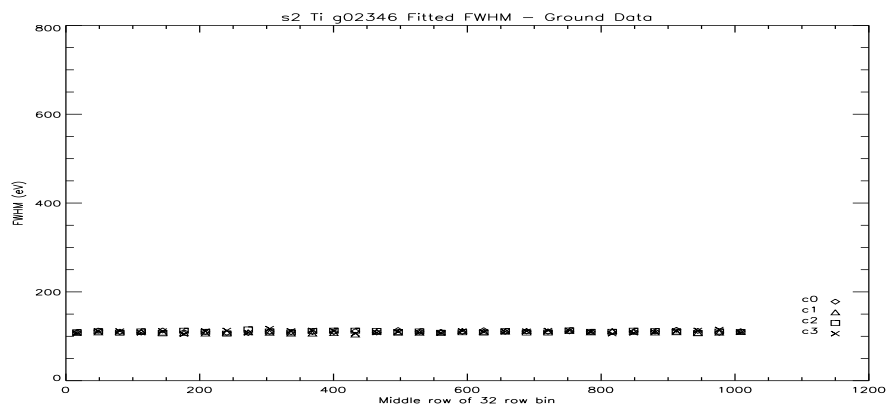
Figure 141: S2 Ti FWHM Vs Row at -110C.
