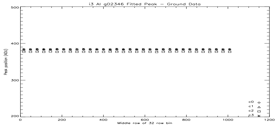
Figure 101: i3 Al Peak Vs Row at -110C.
