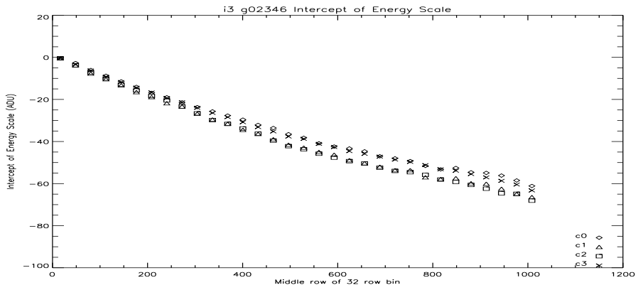
Figure 69: i3 Intercept of the Energy Scale Vs Row at -110C.
