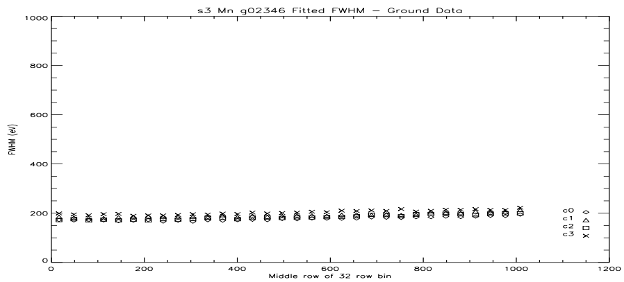
Figure 145: S3 Mn FWHM Vs Row at -110C.
