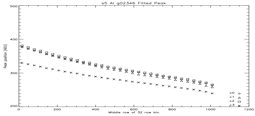
Figure 29: S5 Al Peak Vs Row at -110C.
