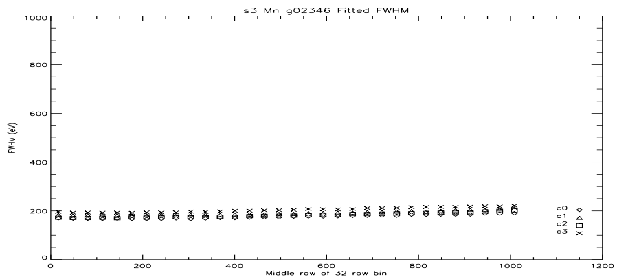
Figure 55: S3 Mn FWHM Vs Row at -110C.
