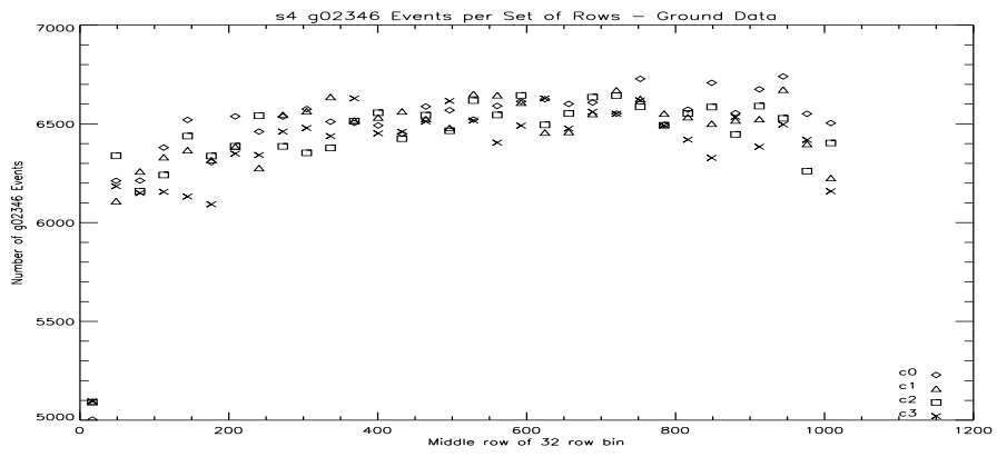
Figure 180: S4 ASCA G02346 Counts Vs Row at -110C.
