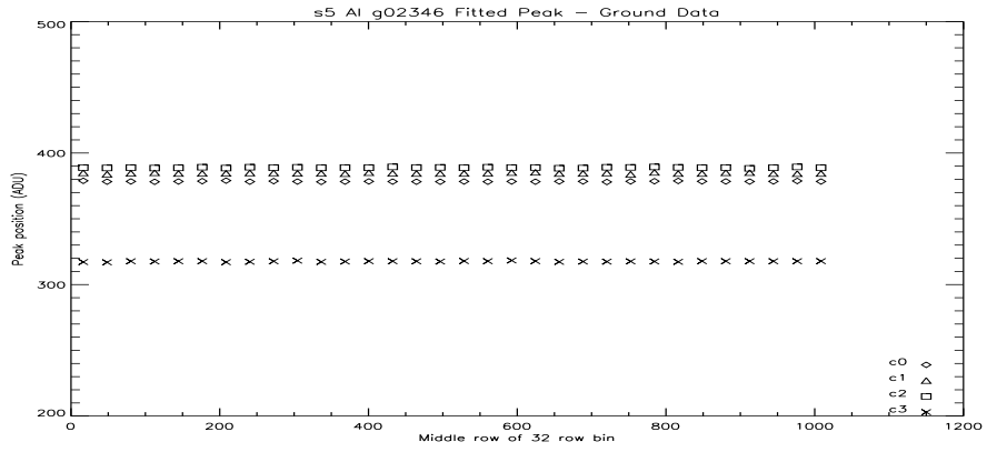
Figure 119: S5 Al Peak Vs Row at -110C.
