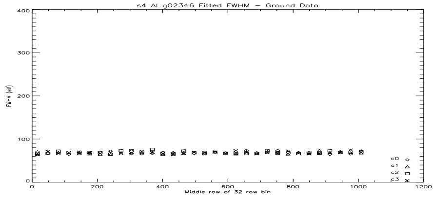
Figure 146: S4 Al FWHM Vs Row at -110C.
