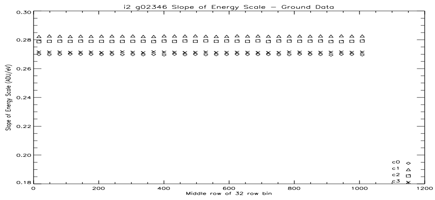
Figure 156: i2 Slope of the Energy Scale Vs Row at -110C.
