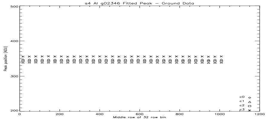
Figure 116: S4 Al Peak Vs Row at -110C.
