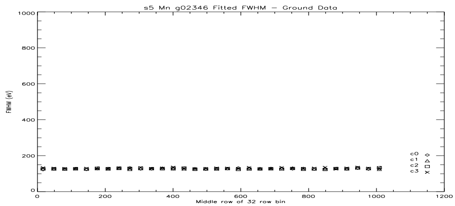
Figure 151: S5 Mn FWHM Vs Row at -110C.
