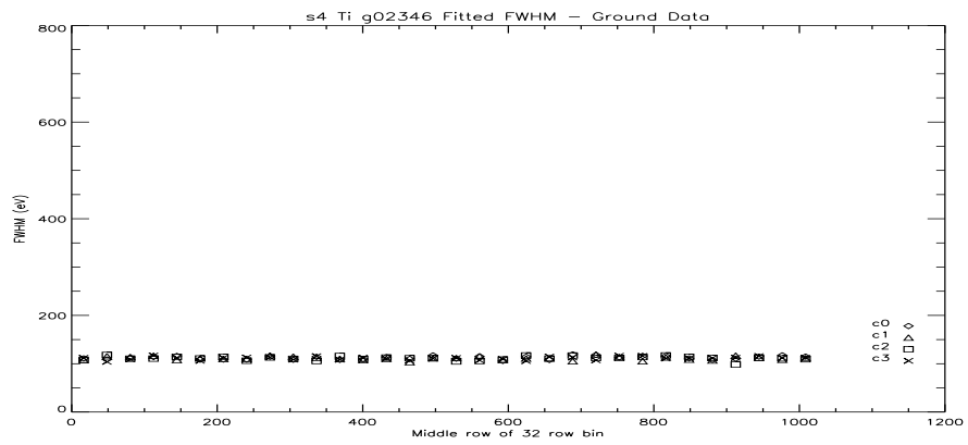
Figure 147: S4 Ti FWHM Vs Row at -110C.
