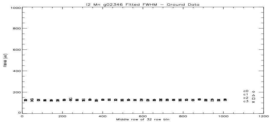
Figure 130: i2 Mn FWHM Vs Row at -110C.
