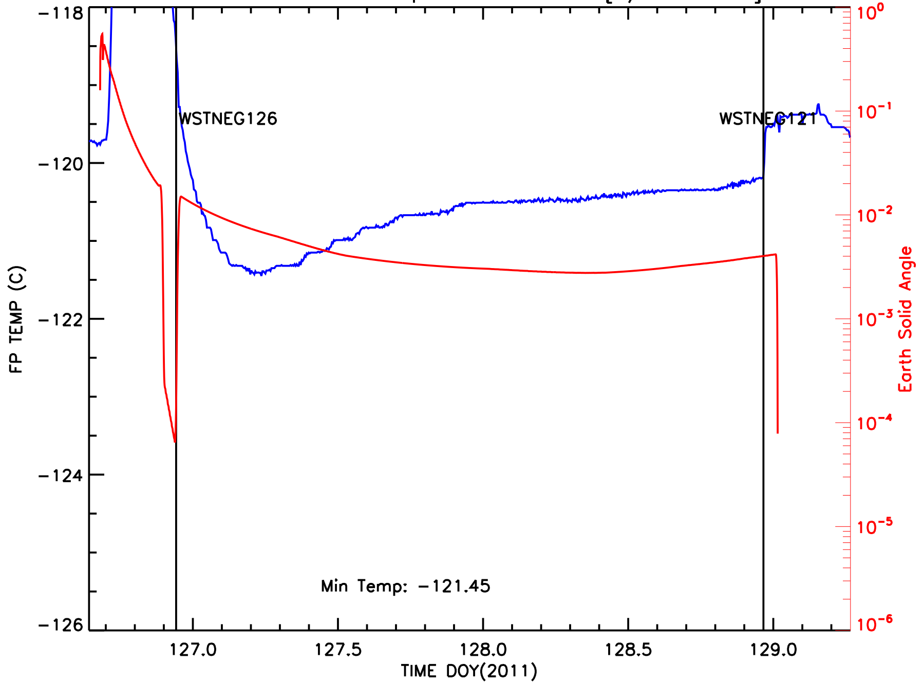
ACIS Focal Plane Temperature vs Time [5/1-3 2011]
