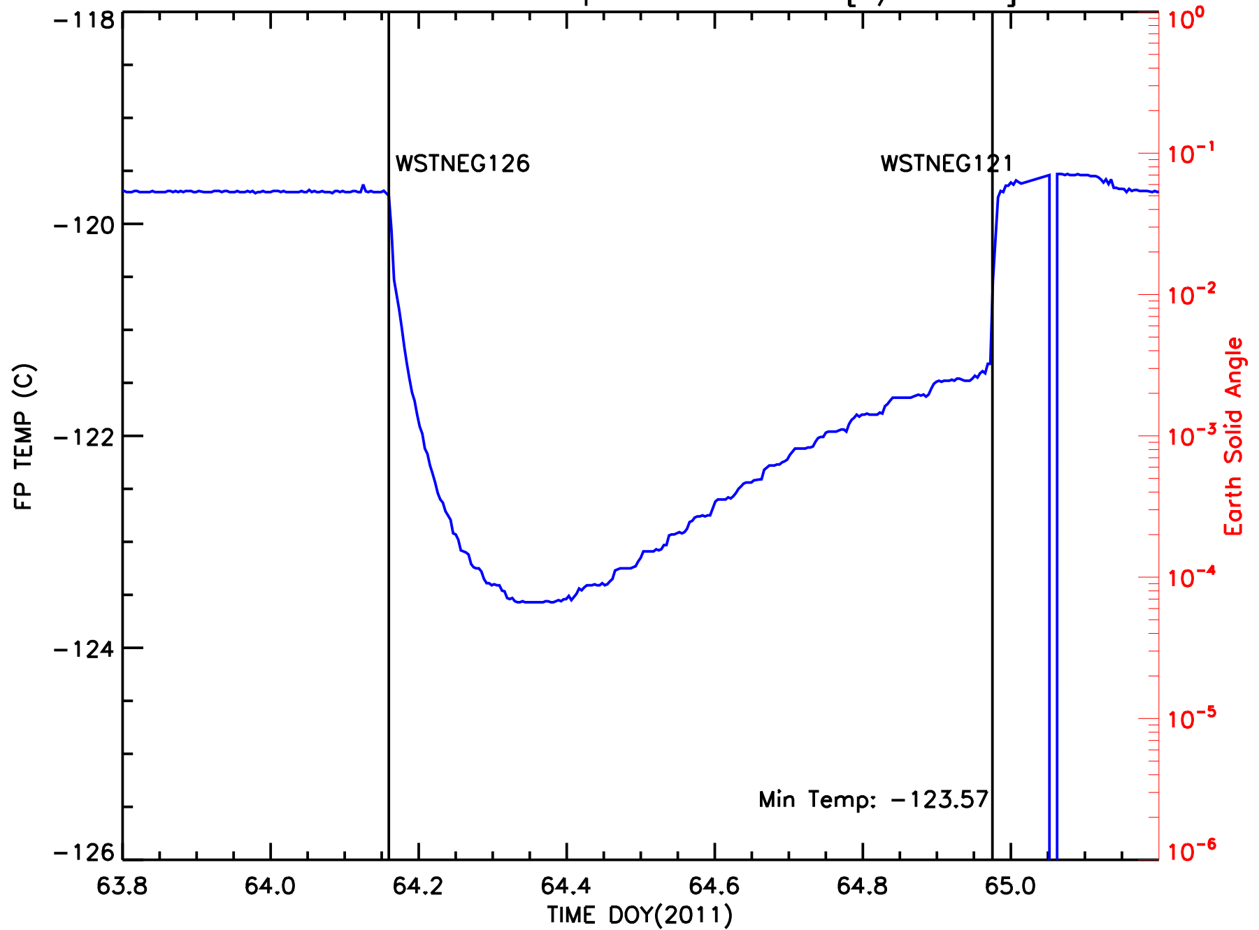
ACIS Focal Plane Temperature vs Time [3/5 2011]
