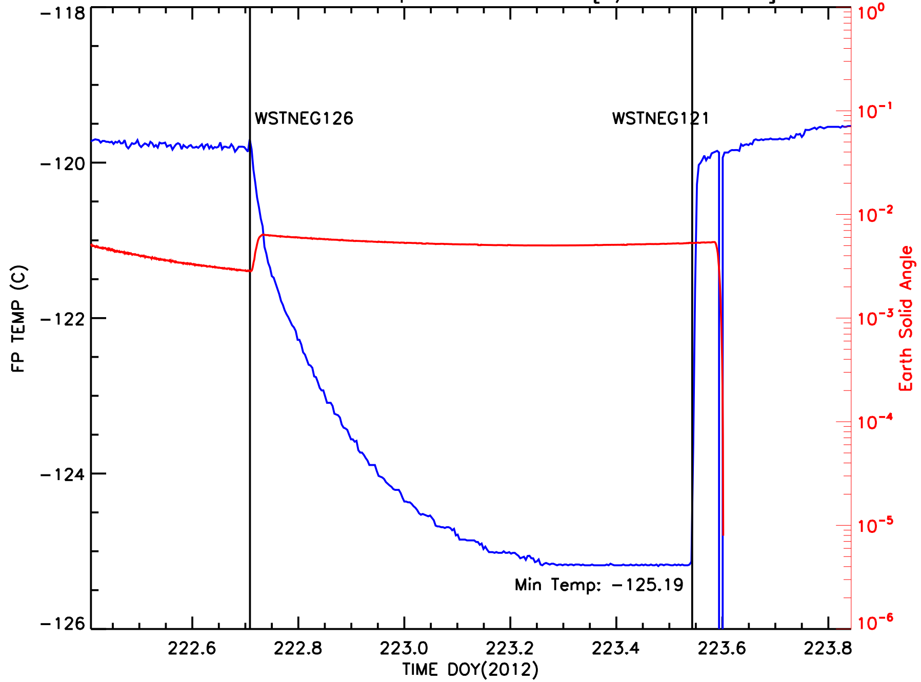
ACIS Focal Plane Temperature vs Time [8/10-11 2010]
