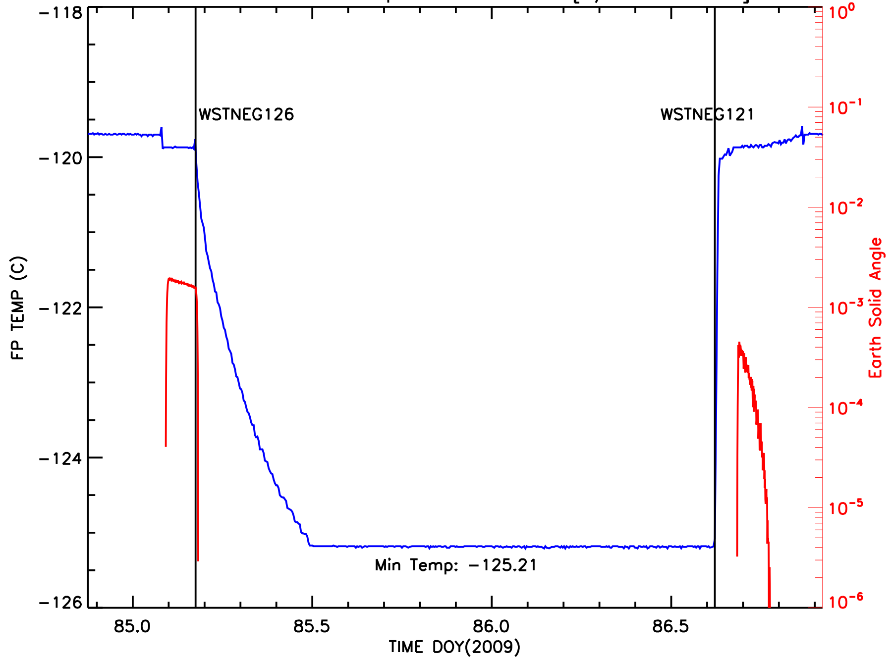
ACIS Focal Plane Temperature vs Time [3/25-26 2009]
