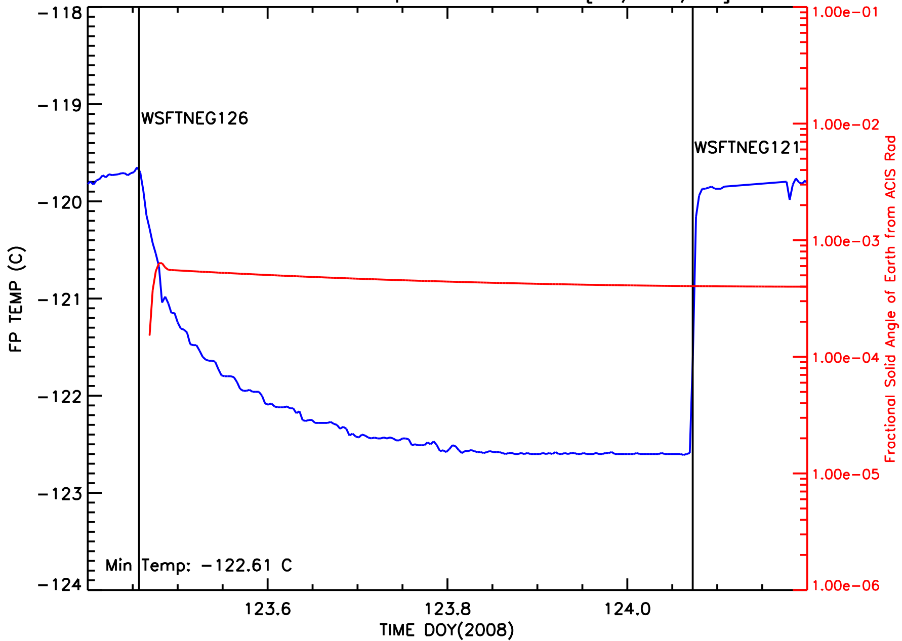
ACIS Focal Plane Temperature vs Time [05/3-4/08]
