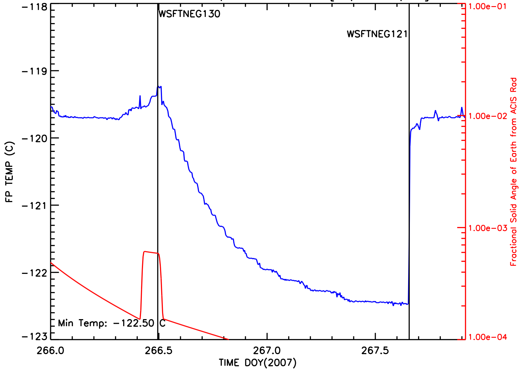
ACIS Focal Plane Temperature vs Time [09/23-25/07]
