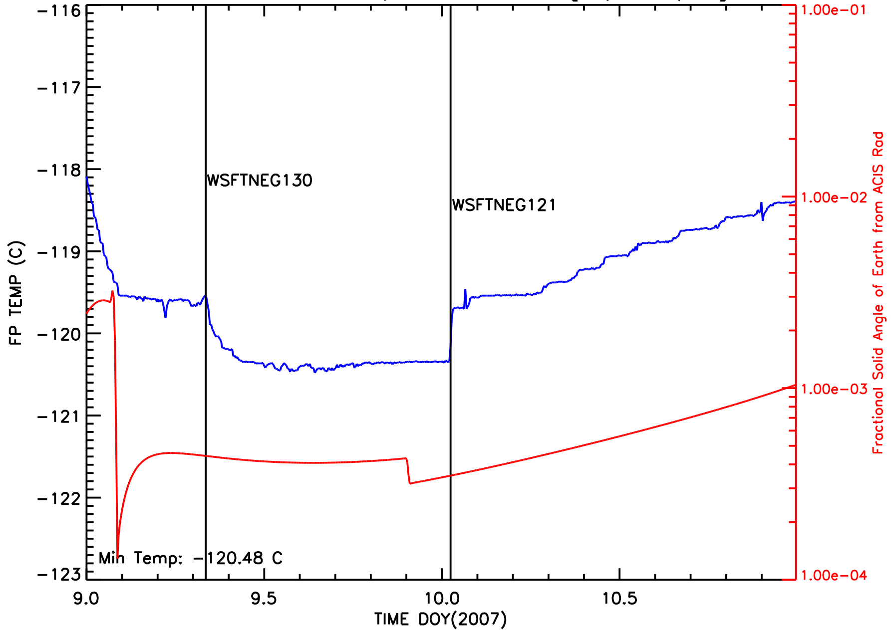
ACIS Focal Plane Temperature vs Time [01/9-11/07]
