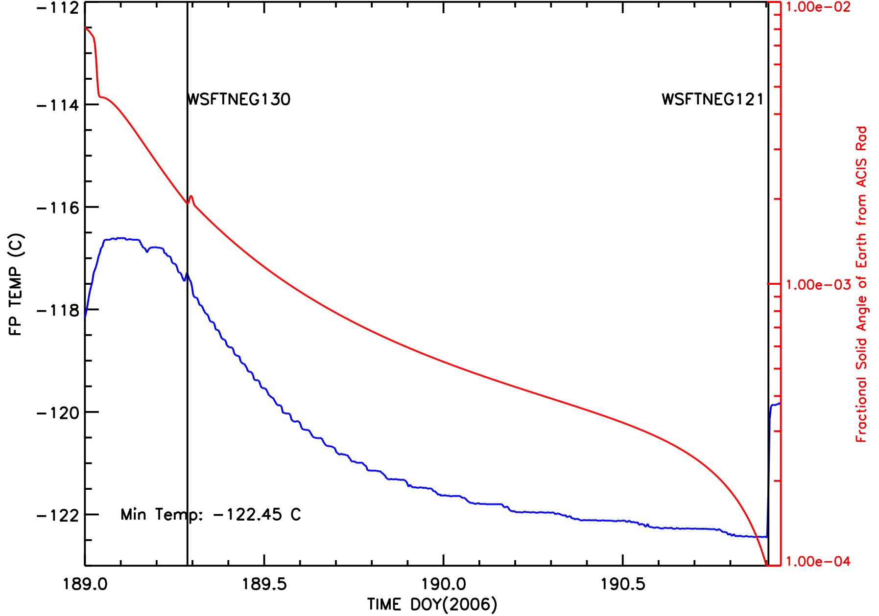
ACIS Focal Plane Temperature vs Time [07/08-09/06]
