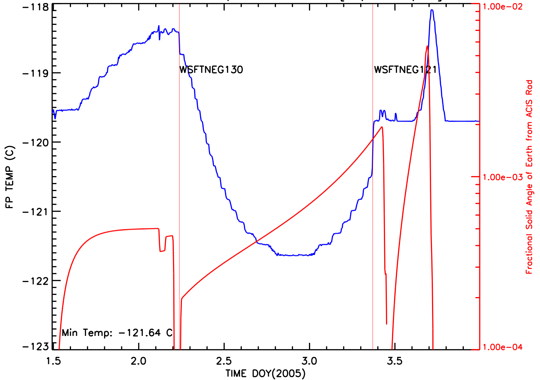
ACIS Focal Plane Temperature vs Time [01/02-04/06]
