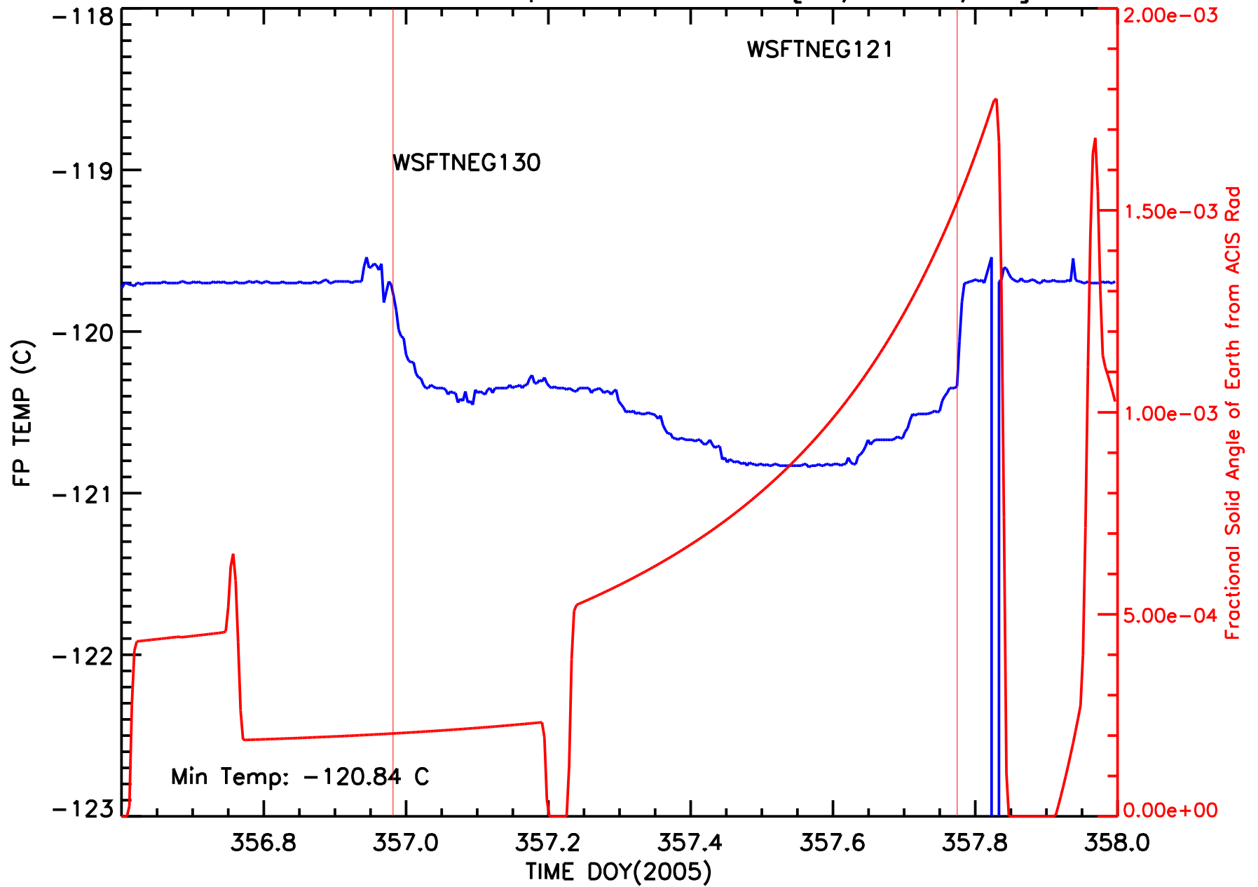
ACIS Focal Plane Temperature vs Time [12/22-24/05]
