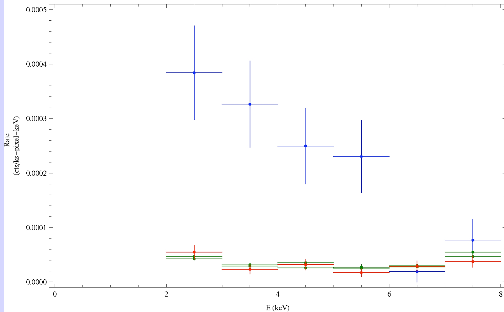
Measured spectra above 2 keV for Northern aurora and background
