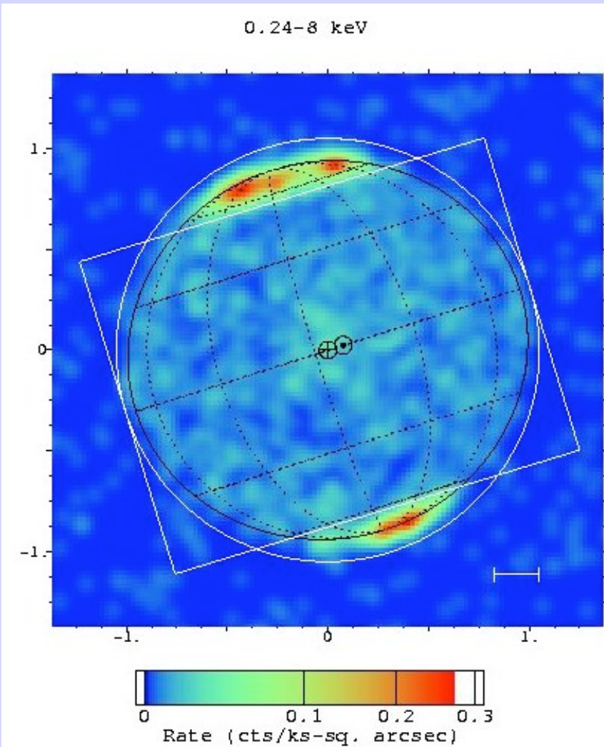
Chandra
