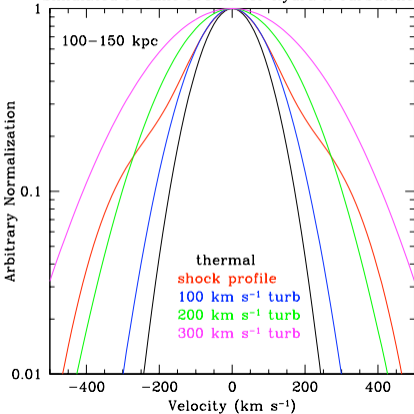
Simulated Fe Line Profile for Hydra A Turbulence
