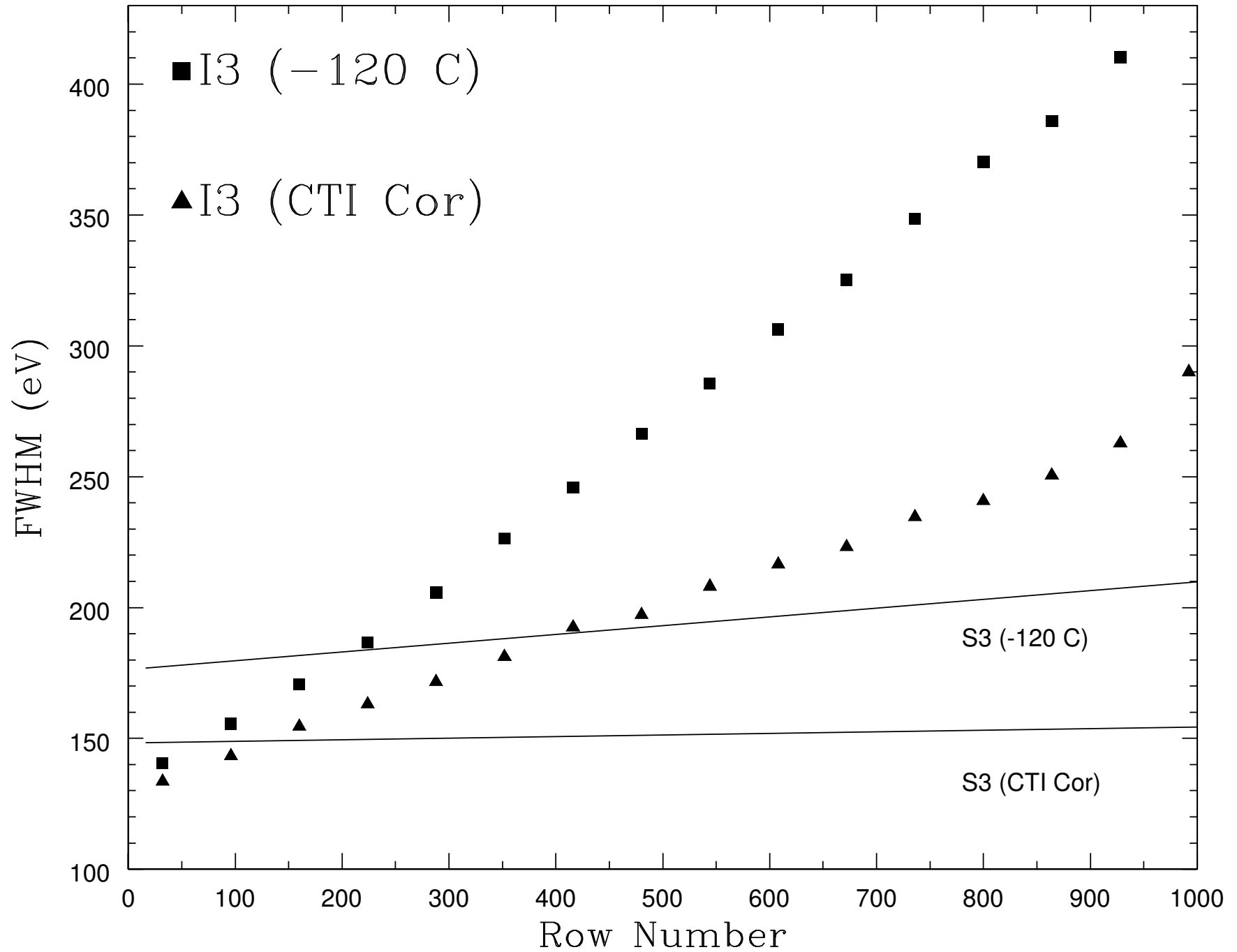
ACIS I3 and S3 FWHM vs Row at Mn-K (OBSID 62895)
