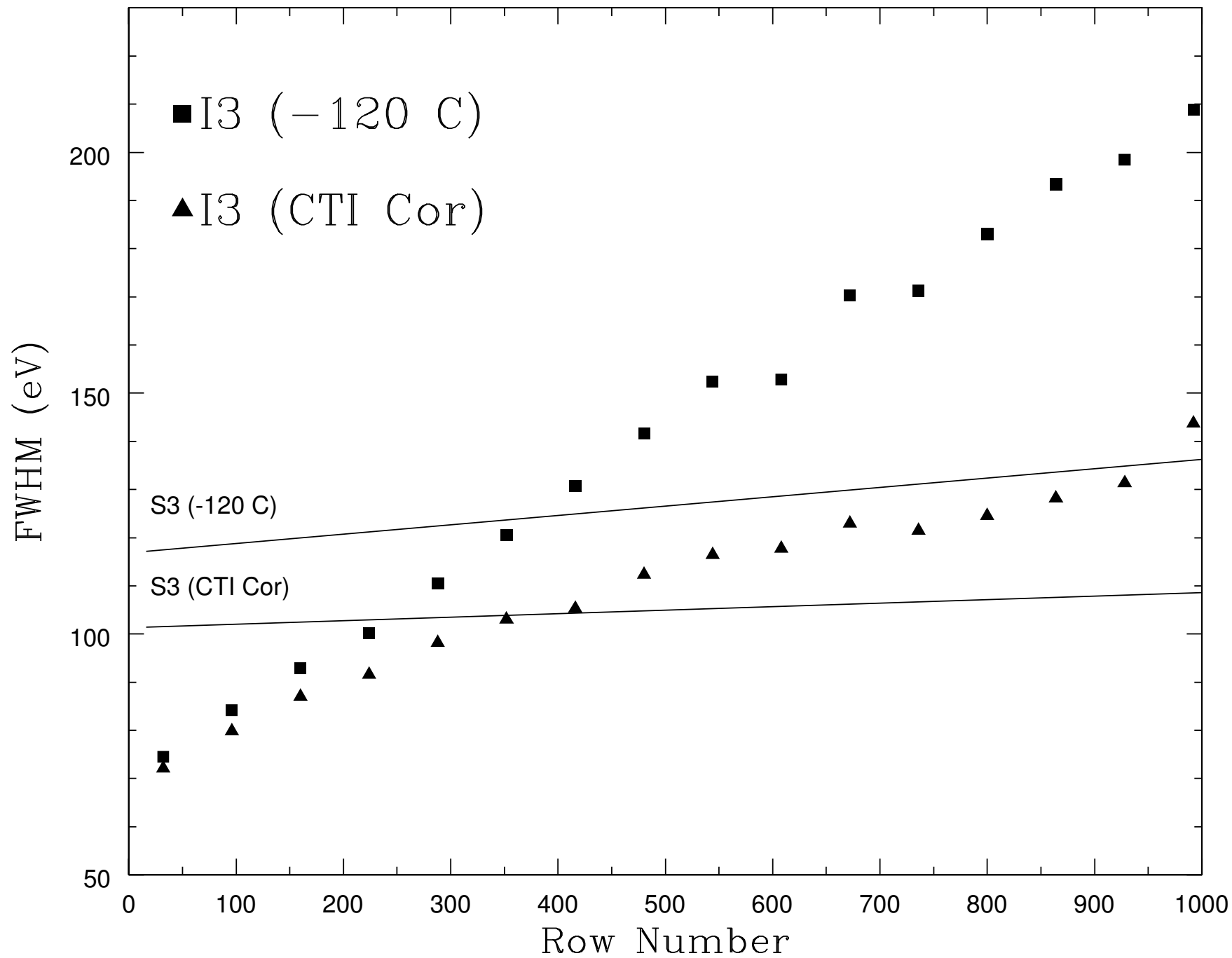
ACIS I3 and S3 FWHM vs Row at Al-K (OBSID 62895)
