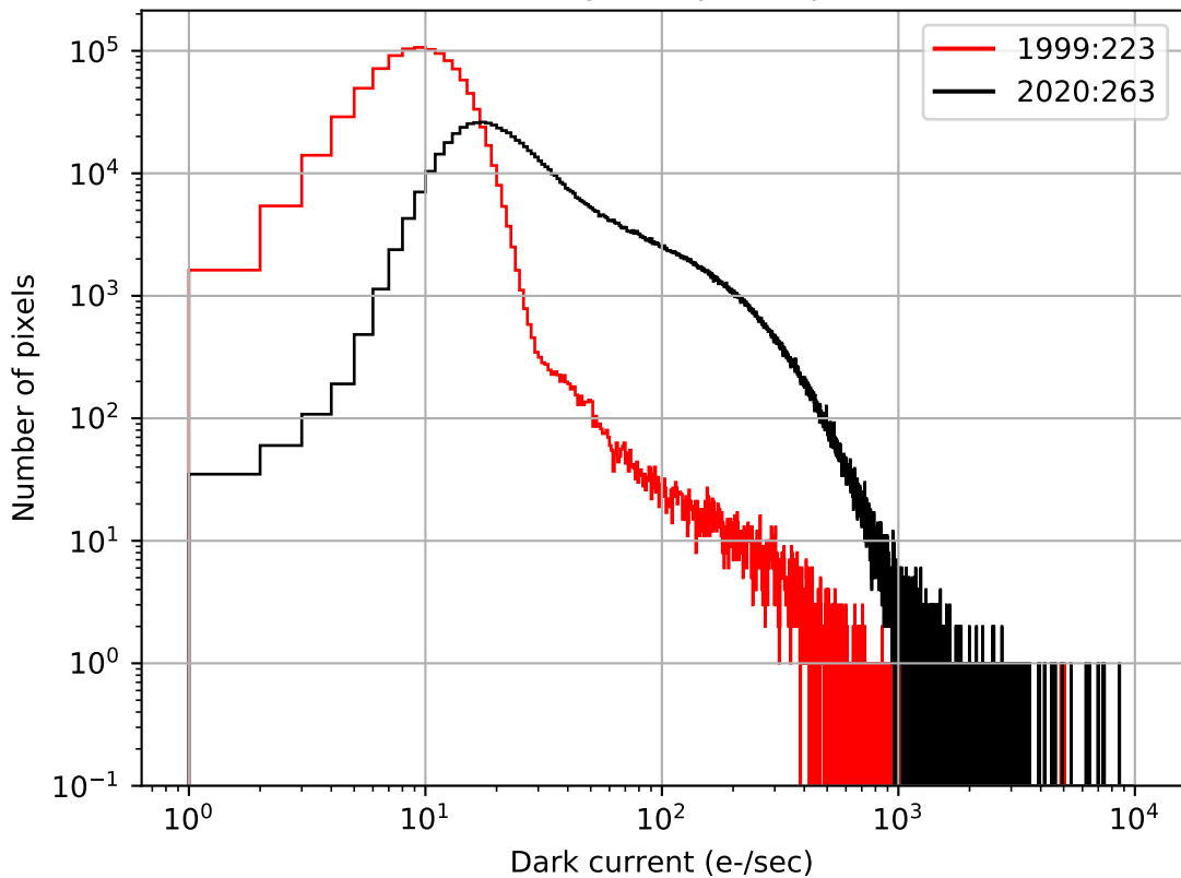
Dark current histogram (pixels per e-/sec bin)
