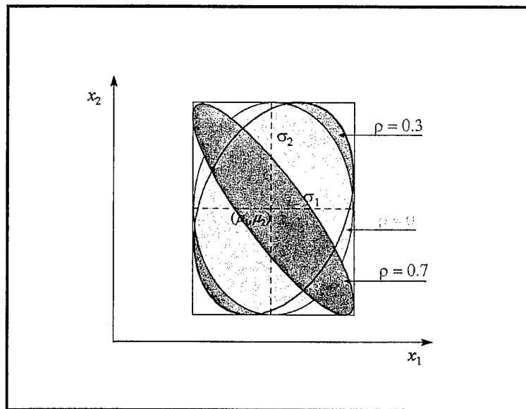
Figure 2.1 COVARIANCE ELLIPSES
