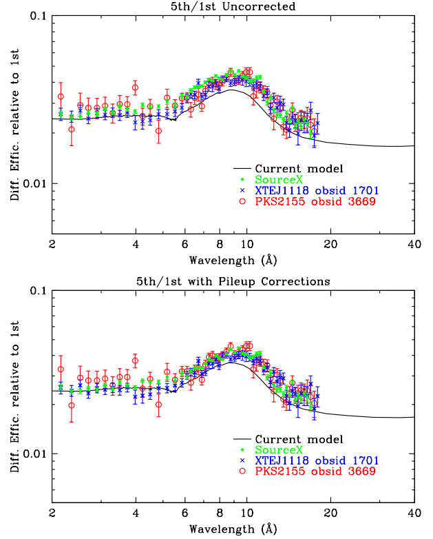
Figure 8. Ratio of 5th and 1st-order efficiencies. Current model appears to be \sim 15\% low at most wavelengths, but the overall agreement in shape is good.
