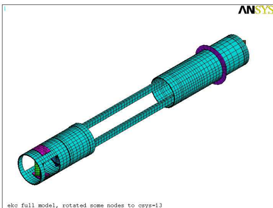
Figure E.8: EKC Solid Model of Fiducial Transfer System Periscope.
