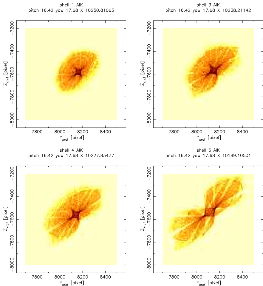
Figure 30.13: Off-axis images for individual shells; pitch = 16.42' , yaw = 17.68' . Pixel width 6.43\ \mu\text{m} ; binned to 8 \times 8 pixels. Two large overlapping lobes and a dense central pincushion can be seen; the light lanes are shadows of the CAP struts. The concentric ridges in the large lobes result from low-frequency surface errors on the mirrors. (Raytrace data; logarithmic stretch)
