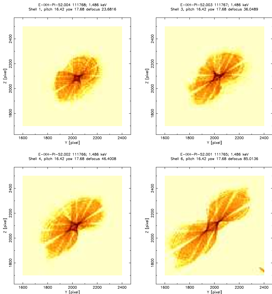
Figure 30.3: Off-axis images for individual shells; pitch = 16.42' , yaw = 17.68' . Pixel width 6.43 \mu\text{m} ; binned to 8 \times 8 pixels. Two large overlapping lobes and a dense central pincushion can be seen; the light lanes are shadows of the CAP struts. The concentric ridges in the large lobes result from low-frequency surface errors on the mirrors. (X-ray data; logarithmic stretch)
