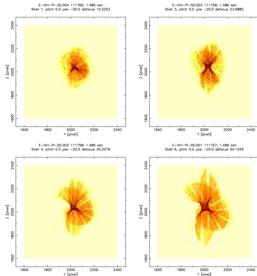
Figure 30.2: Off-axis images for individual shells; pitch = 0' , yaw = -20' . Pixel width 6.43 \mu\text{m} ; binned to 8 \times 8 pixels. Two large overlapping lobes and a dense central pincushion can be seen; the light lanes are shadows of the CAP struts. The concentric ridges in the large lobes result from low-frequency surface errors on the mirrors. (X-ray data; logarithmic stretch)
