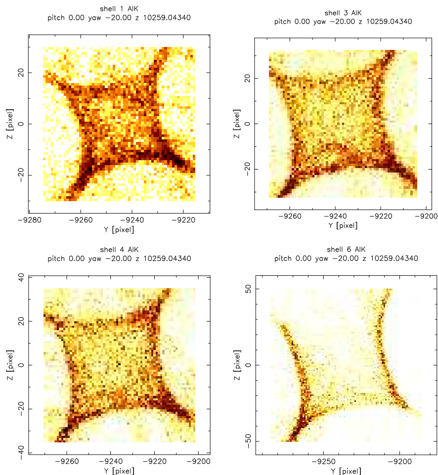
Figure 30.10: Core pincushions of off-axis images for individual shells based on current SAO raytrace model; pitch = 0' , yaw = -20' . Pixel width 6.43\ \mu\text{m} ; binned to 1 \times 1 pixels. (Raytraced; logarithmic stretch)
