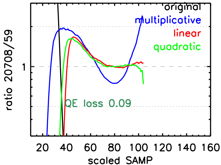
2018-07-28T13:28:05 Offaxis=0.2 arcmin
