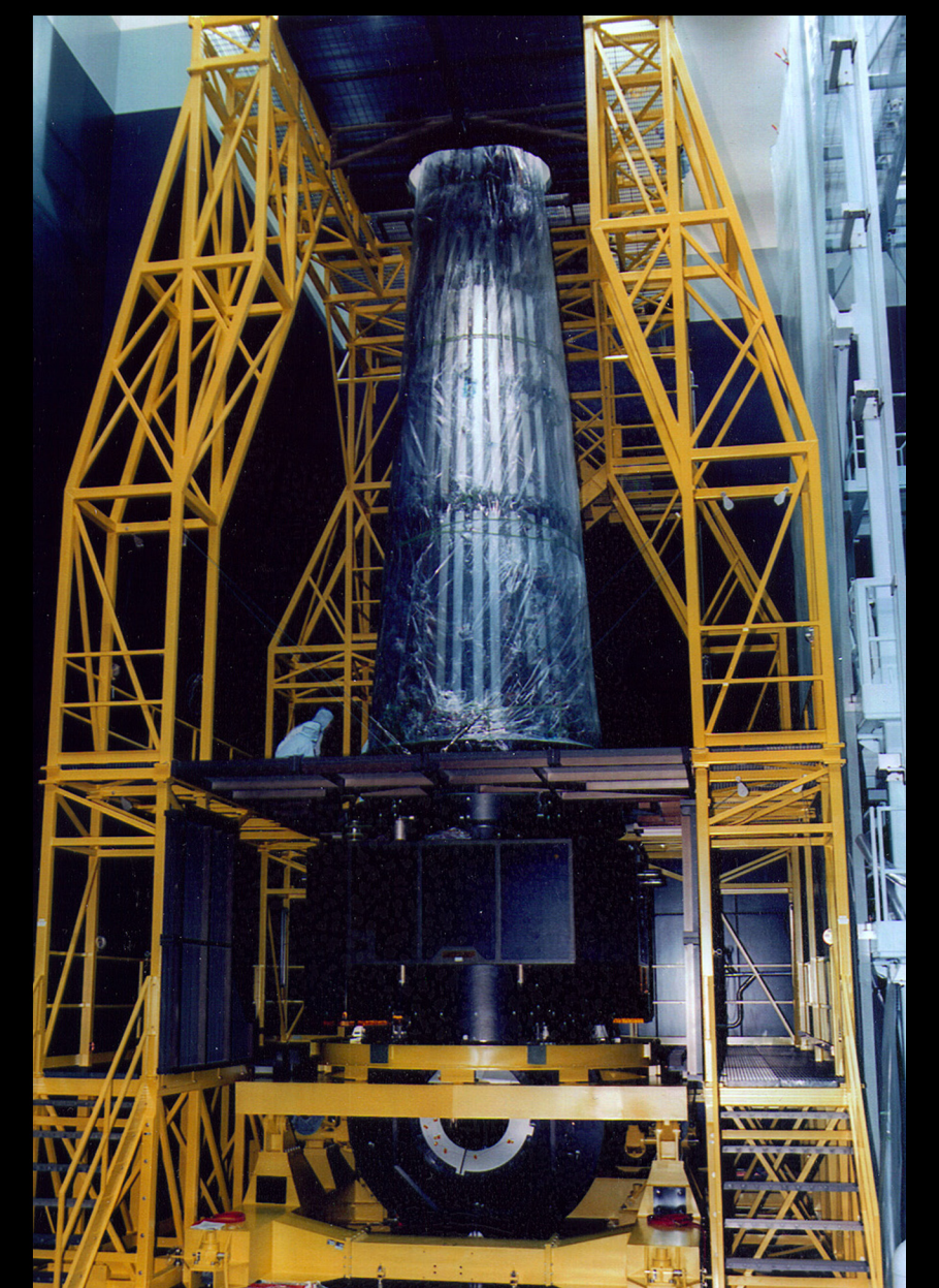
System ready for modal survey
