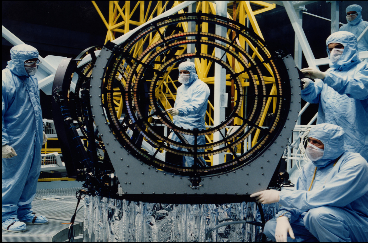
Optical Transmission Grating (OTG) Installation at Northrop Grumman Aerospace Systems (NGAS)
